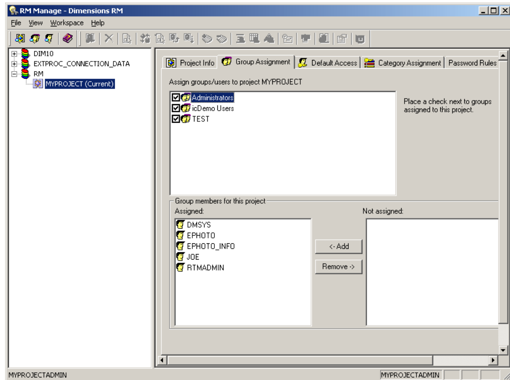
Figure 1-5. RM Manage
