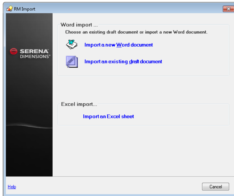
Figure 1-3. RM Import
