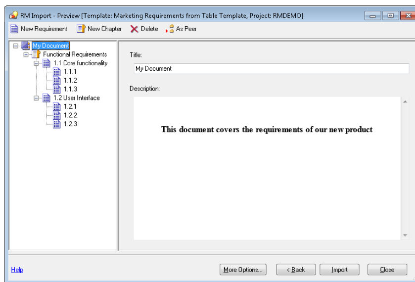
Figure 5-4. Preview Dialog
