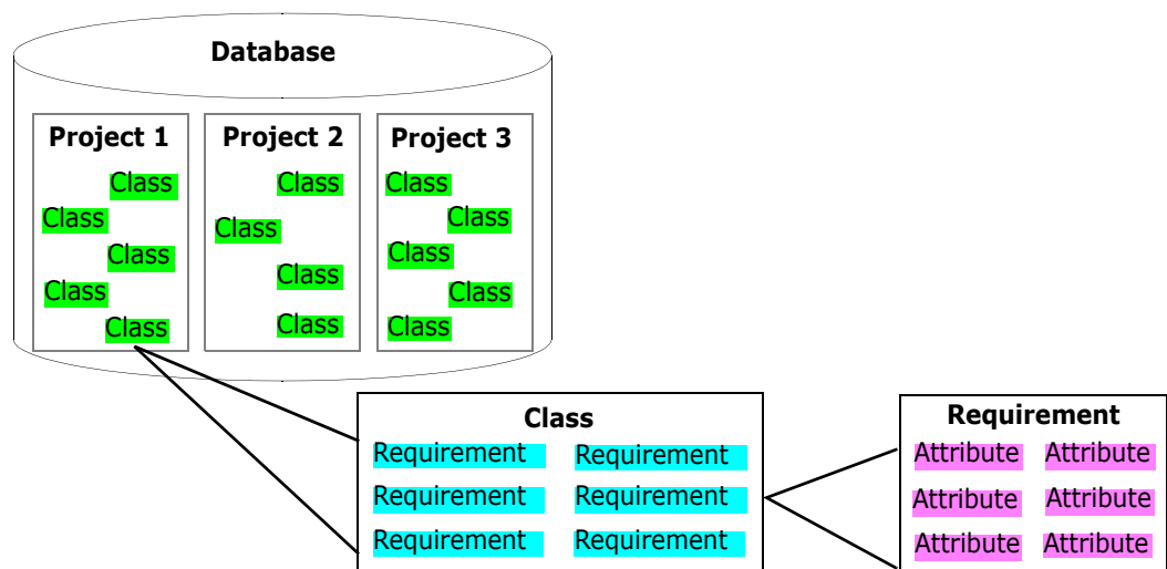
Figure 1-7. Dimensions RM Data Structure
