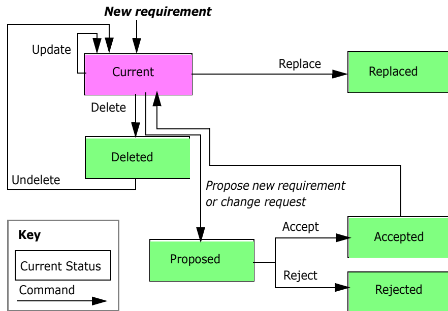
Figure 1-9. Object Lifecycle
