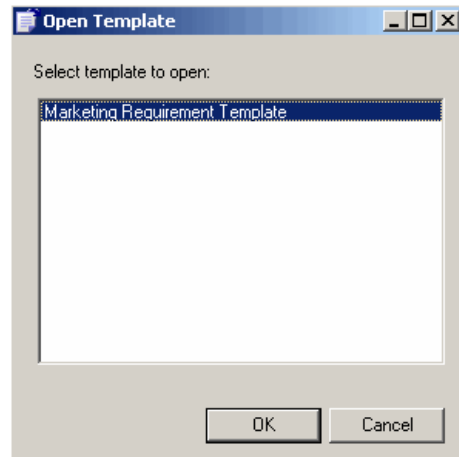
Figure 6-2. Open Template
