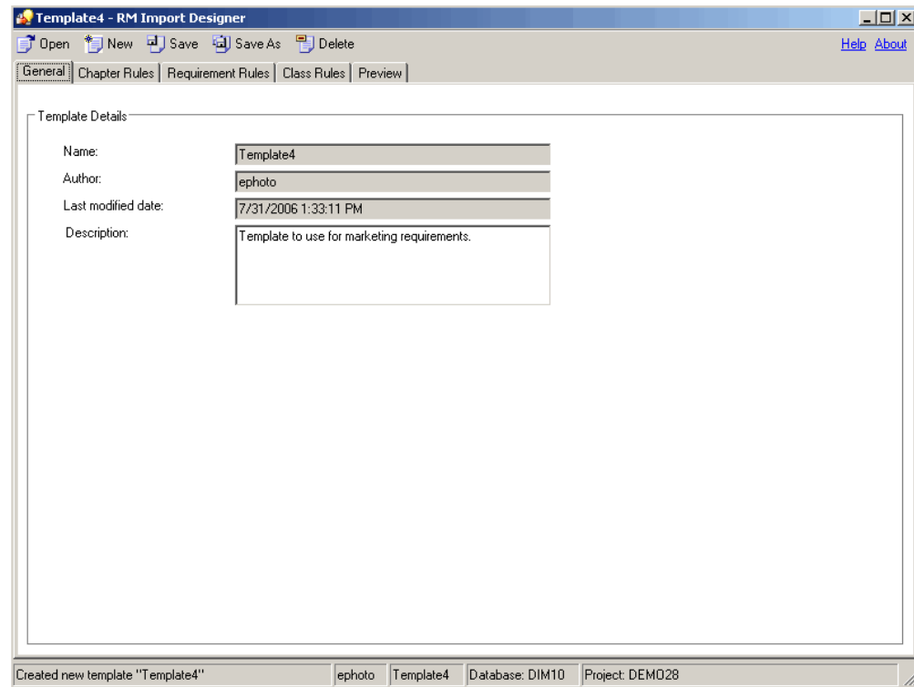
Figure 6-4. General Tab
