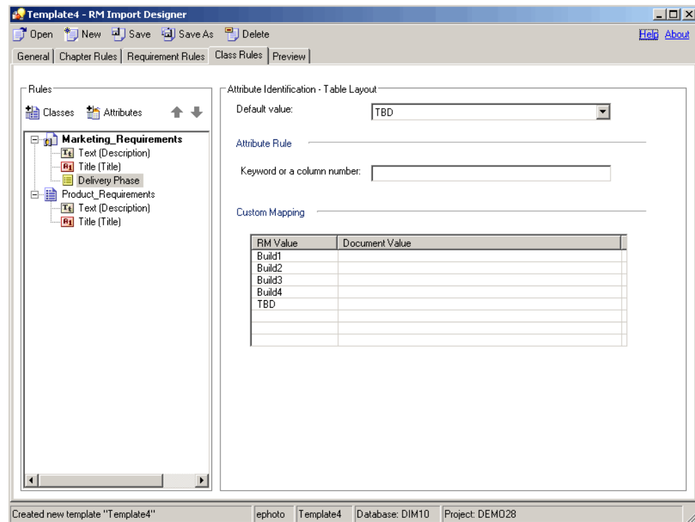
Figure 6-18. Class Rules Tab—Table Layout—List Attributes
