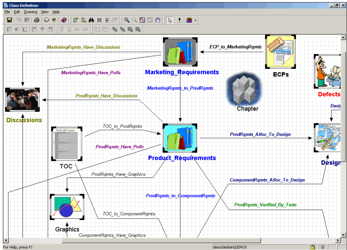
Figure 1-6. Class Definition
